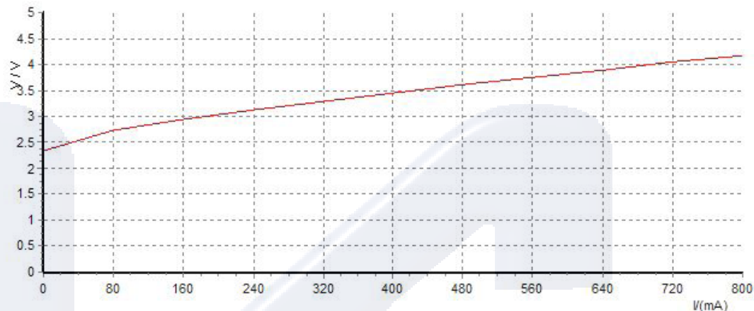
I-V curve
