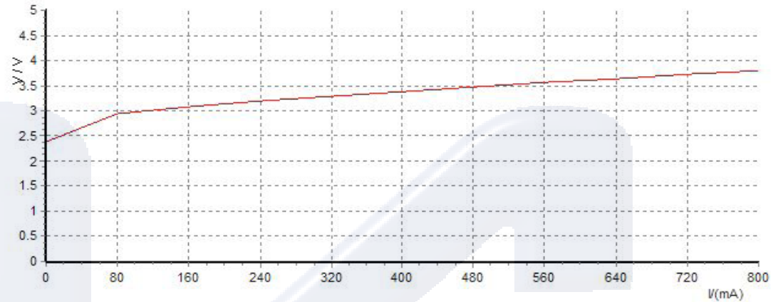
I-lcurve
