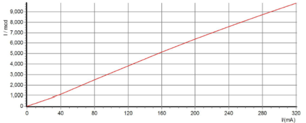
I-l curve
