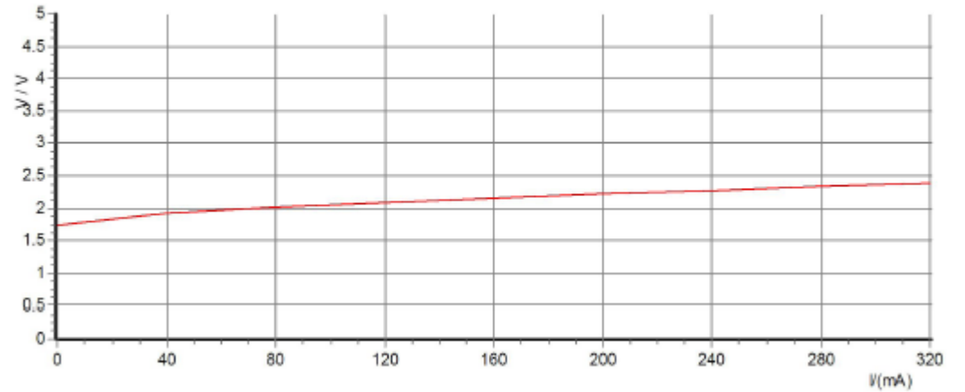
I-l curve
